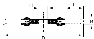
Form 1RDZ
