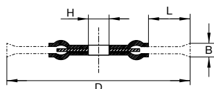
Form 1RDZ
