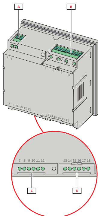
Fig. 2 Bagside
