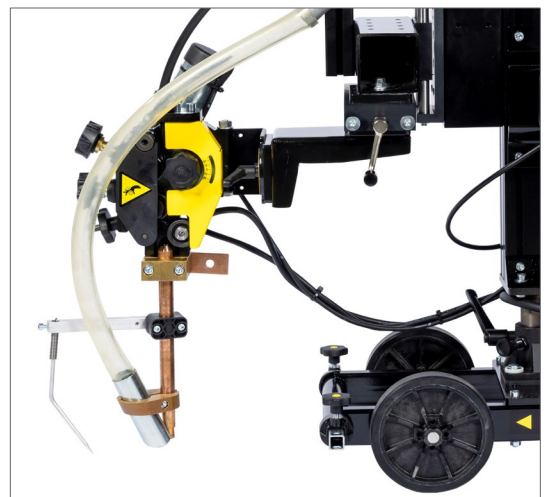
The intelligent memory function ensures perfect wire feed before and after wire spool changes.
