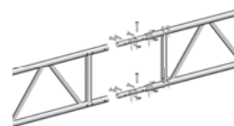
Coupler connection as in sketch possible for Ref. No. 4904
