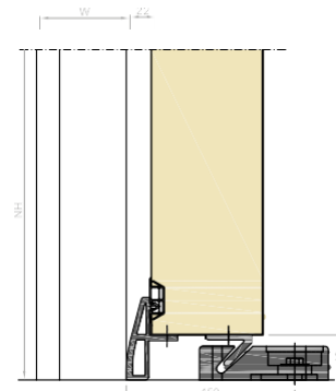
DETAIL 4: +°C
