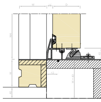
DETAIL 4: -°C
