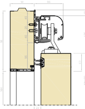
DETAIL 3: +°C
