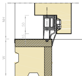
DETAIL 4: -°C
