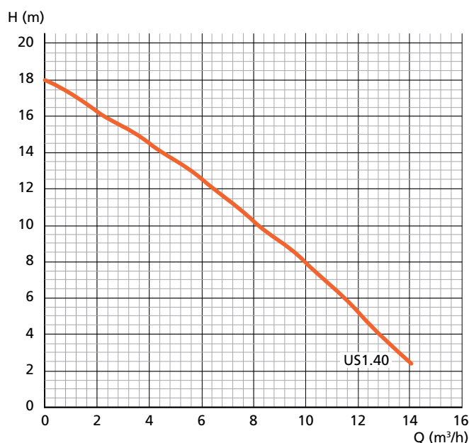
mini-Compacta US1.40 characteristic curve
