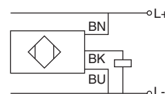
connection amplifier
