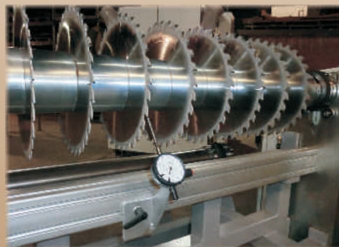
Balancing system for the tool-holder shafts
