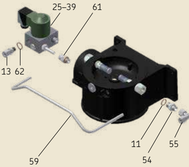
SKF MonoFlex layout B with two pump elements
