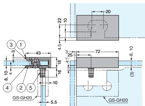
Drawing shows left side installation
