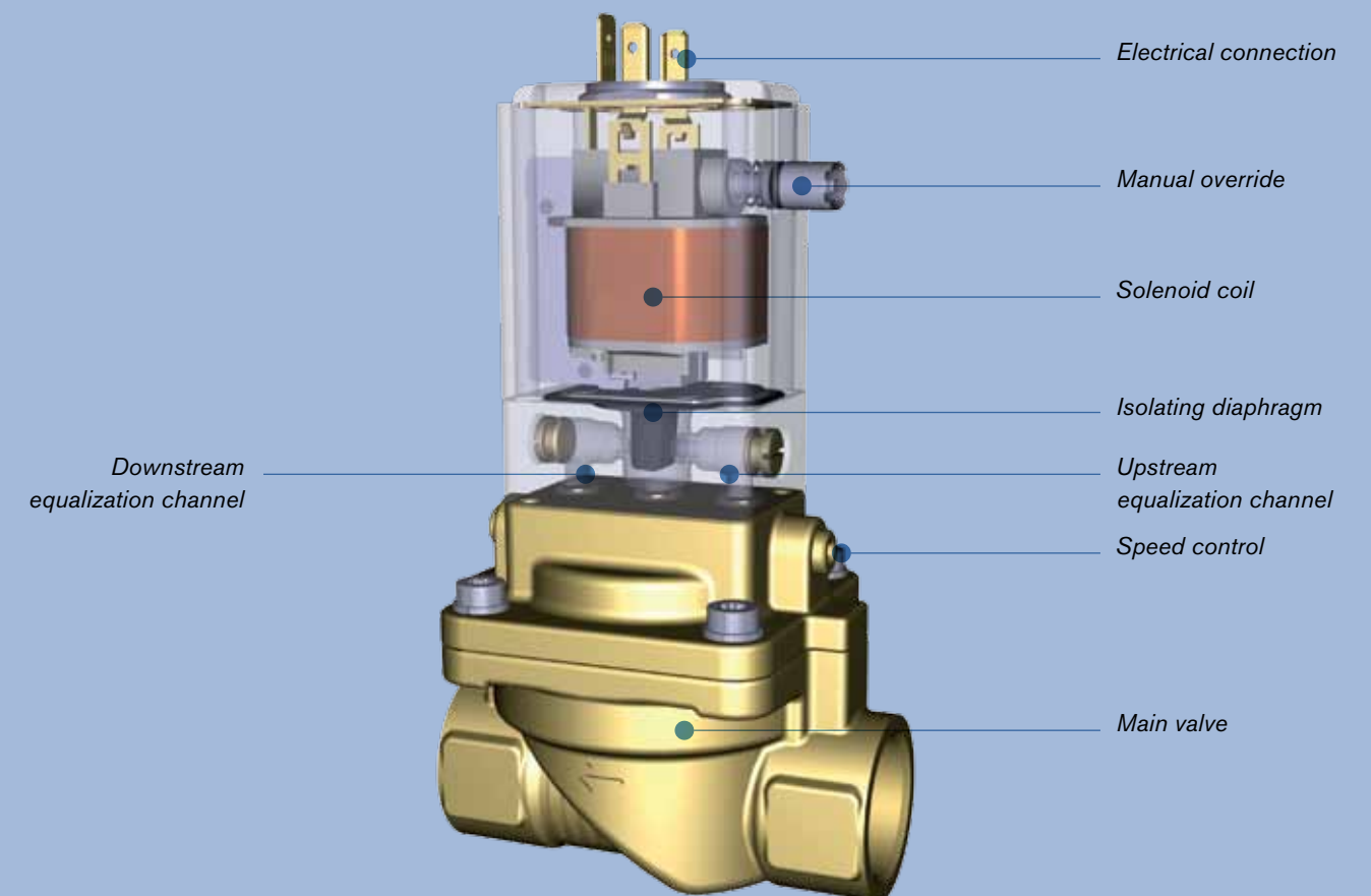
Servo assisted solenoid valve with 3/2-way pilot type 5282
