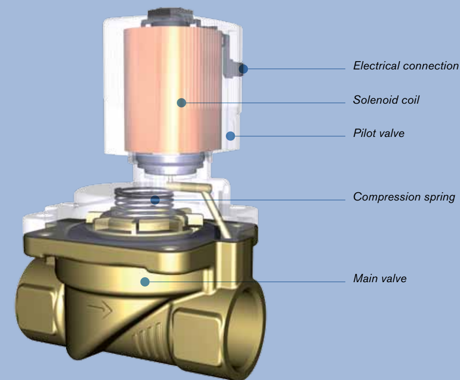
Servo assisted solenoid valve with diaphragm type 6281EV
