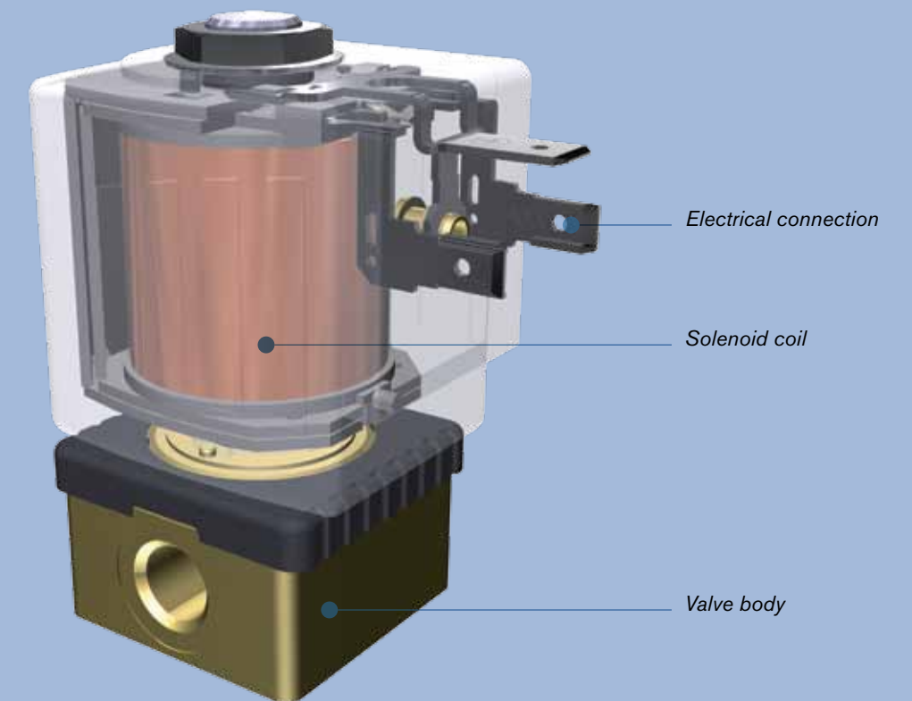
2/2-way plunger-type solenoid valve type 6013
