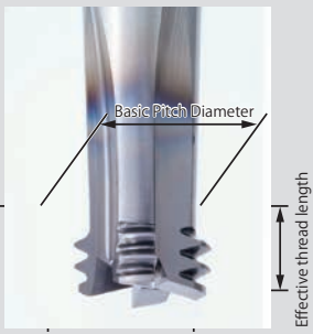
Processing by thread mill
