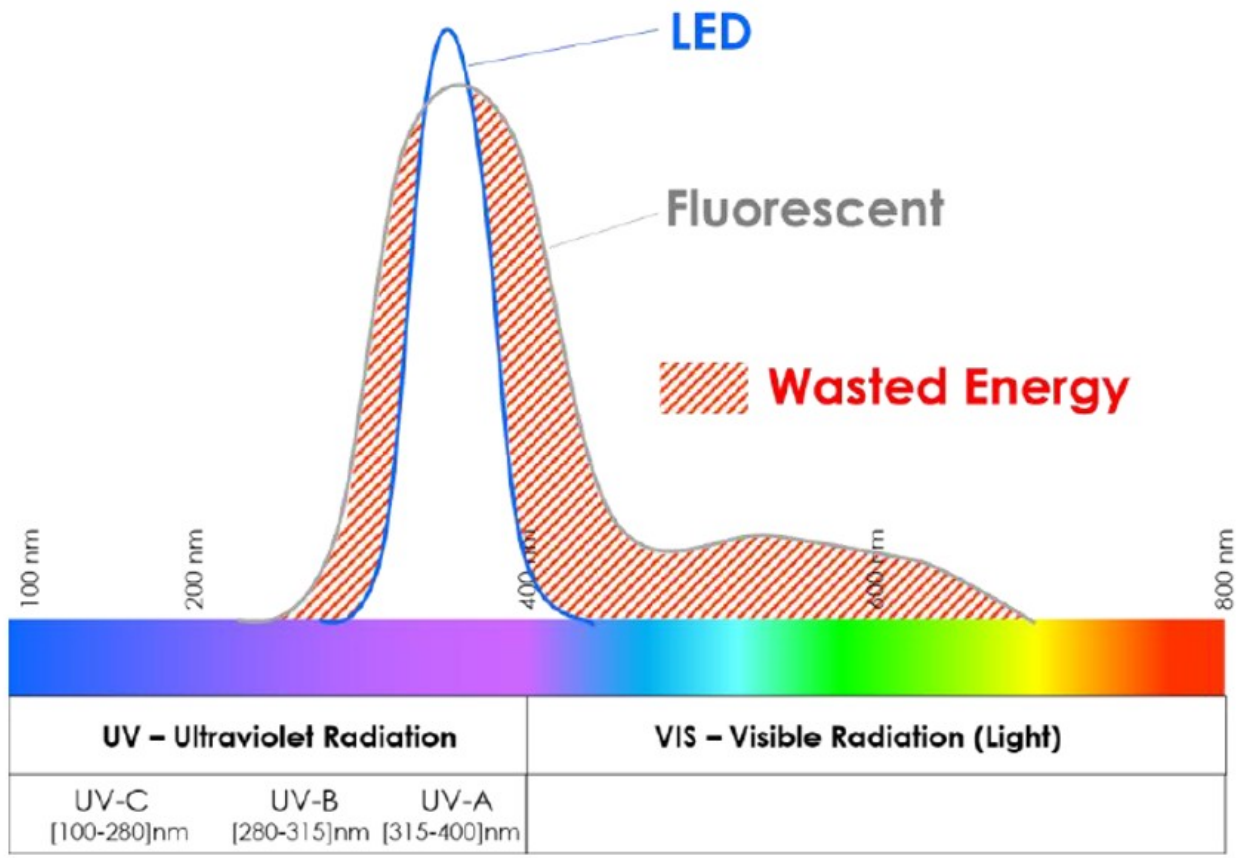
Figure 1 - Comparison of UVA Irradiance Between Fluorescent and LED Sources
