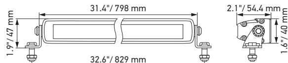
Black Magic Lightbar 32" (Slim)
