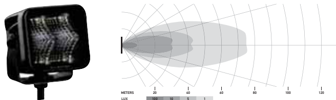
LED Cube SET 2,7", bred lysfordeling
