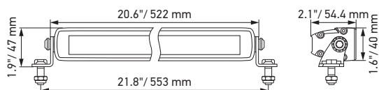
Black Magic Lightbar 20" (Slim)
