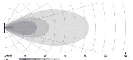
LED Cube SET 3,2", bred lysfordeling
