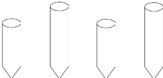
Size 1 Size 2 Size 3 Size 4 Diameter: 18cm Length: 45 cm Flow: 380 l/min Diameter: 18cm Length: 85 cm Flow: 680 l/min Diameter: 10cm Length: 25 cm Flow: 100 l/min Diameter: 10cm Length: 40 cm Flow: 150 l/min
