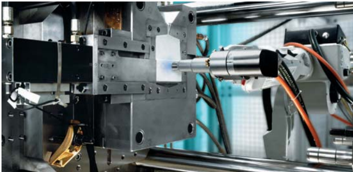
Openair® Plasma pretreatment in two-component injection moulding
