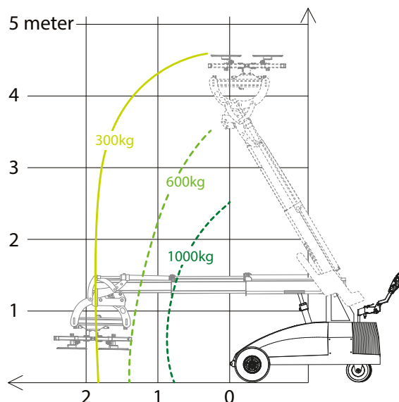
LASTDIAGRAM - VANDRETTE SUGEKOPPER
