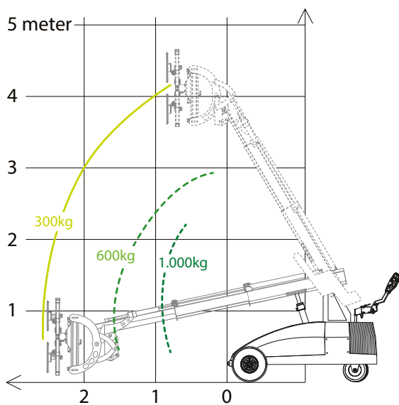
LASTDIAGRAM - LODRETTE SUGEKOPPER
