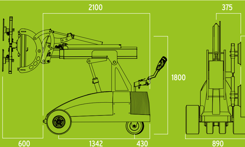
LASTDIAGRAM - VANDRETTE SUGEKOPPER
