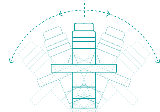
T29 Flex Tilting arbor spindle moulder
