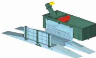
Kit Mobile C (scraper conveyor)
