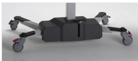
TR 2000 Hydraulisk – Bagsiden af understel
