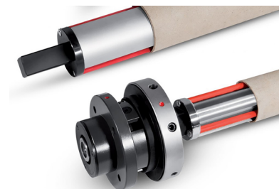
Safety chucks Secures core shafts in place and guarantees roll security during winding processes.
