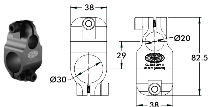
Ø30mm to Ø20mm Cross Clamp
