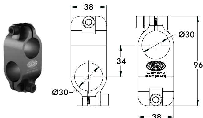
Ø30mm to Ø30mm Cross Clamp
