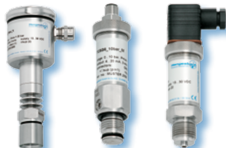
Overload resistant pressure transmitter TCS / TCF... , flush mounted, G 1/2 and M22 x1,5
