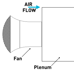
Direct Discharge into Plenum, No Diffuser
