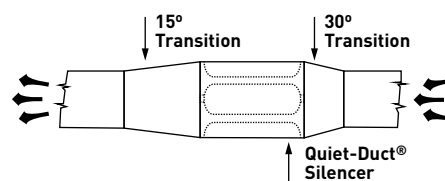
Silencer between Upstream and Downstream Transitions
